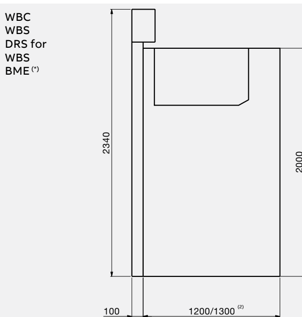
Side view of switchgear with withdrawable circuit-breakers, IAC A-FLR 25 kA, 1 sec up to 17.5 kV and IAC A-FLR 21 kA, 1s at 24 kV with duct
