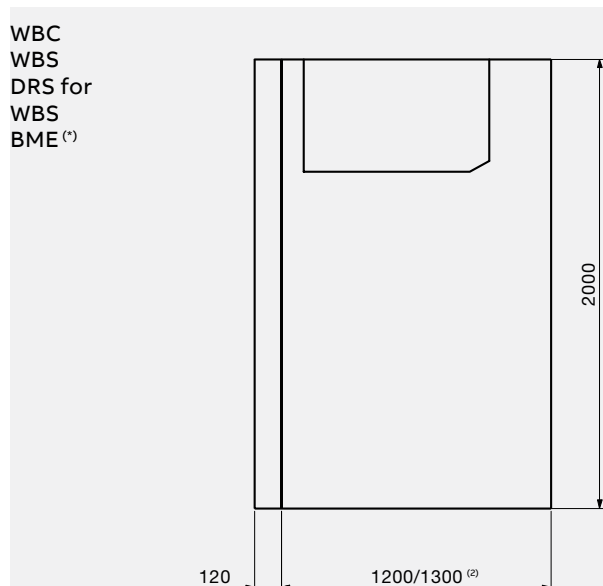
Side view of switchgear with withdrawable circuit-breakers, IAC A-FLR 25 kA, 1 sec up to 17.5 kV and IAC A-FLR 16 kA, 1s at 24 kV with filters
